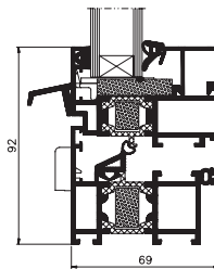
window – cross-section MB-60HI
