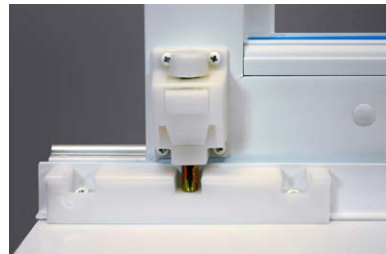
Three-position foot lock option (Only available in white)
